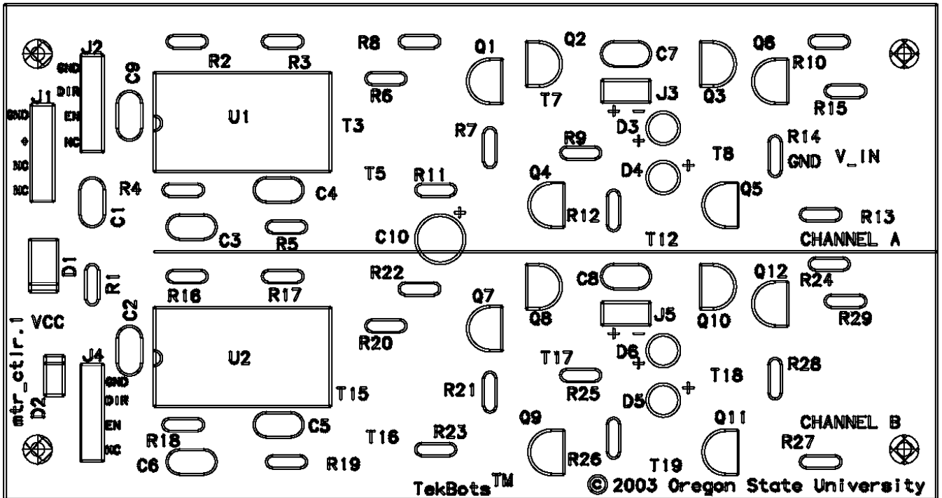
Figure 9.3: Silk Screen of the Motor Controller Board
