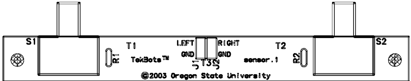
Figure 9.2: Silk Screen of the Sensor Board
