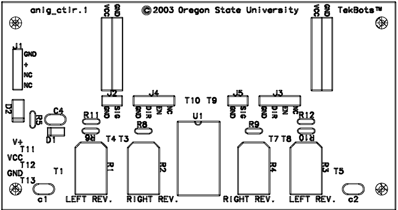
Figure 9.4: Silk Screen of the Analog
