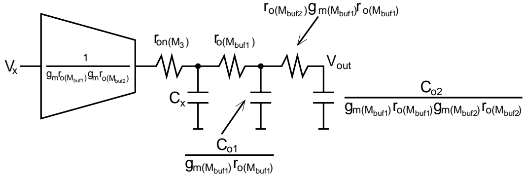
FIGURE 2.18. Small-signal equivalent circuit of new charge pump.
