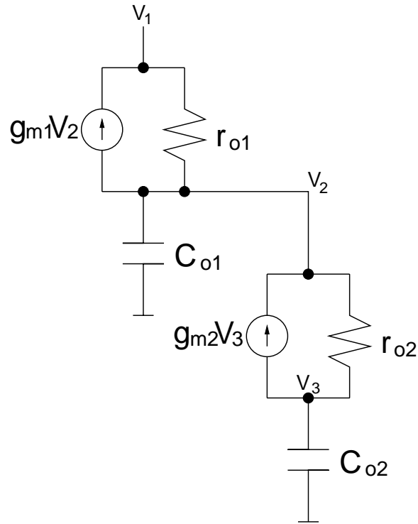
FIGURE E.2. Small-signal model of two cascaded buffer transistors with two output capacitors.
