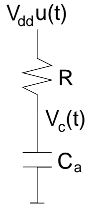
FIGURE B.1. Charging of capacitor C_a to V_{dd} through resistor R .
