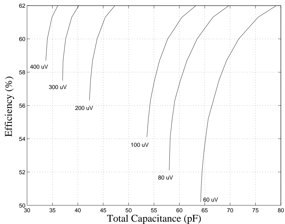
FIGURE 2.15. Total capacitance vs. efficiency for fixed output ripple ( I_o=50 \mu A ).
