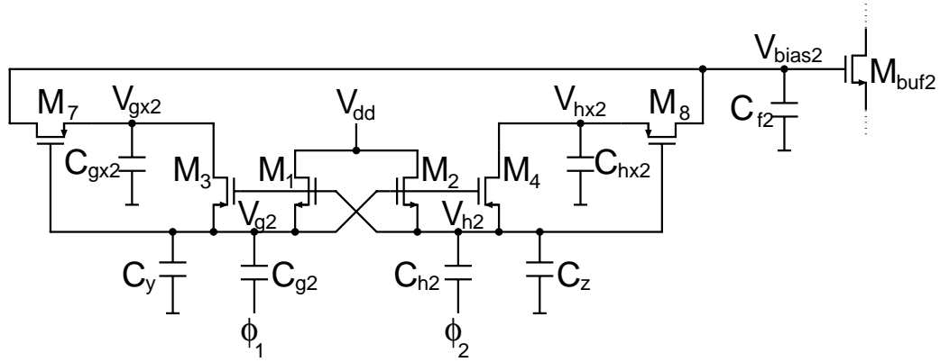
FIGURE 2.17. Conventional charge pump with added capacitors to obtain the second bias voltage.
