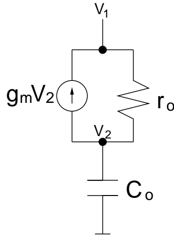
FIGURE E.1. Small-signal model for a single buffer transistor and output capacitor.
